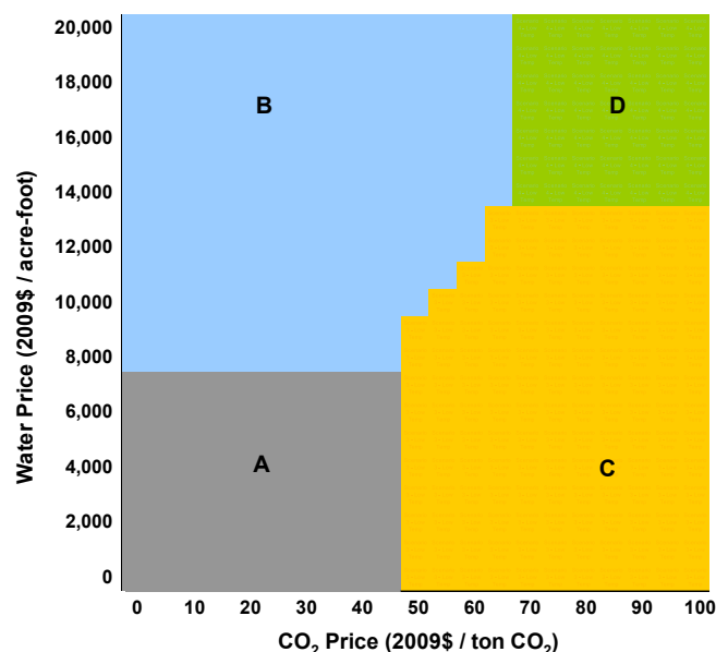
Fig. 2. Least-cost scenarios, without efficiency measures.
