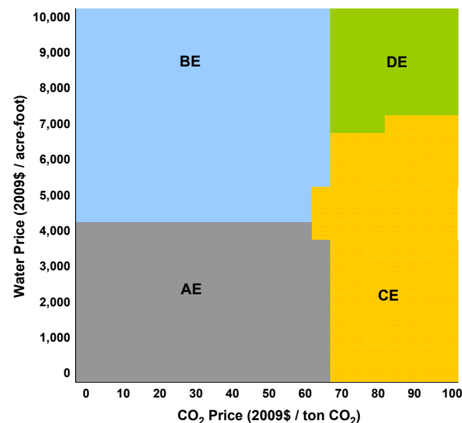
Fig. 3. Least-cost scenarios, with efficiency measures.
